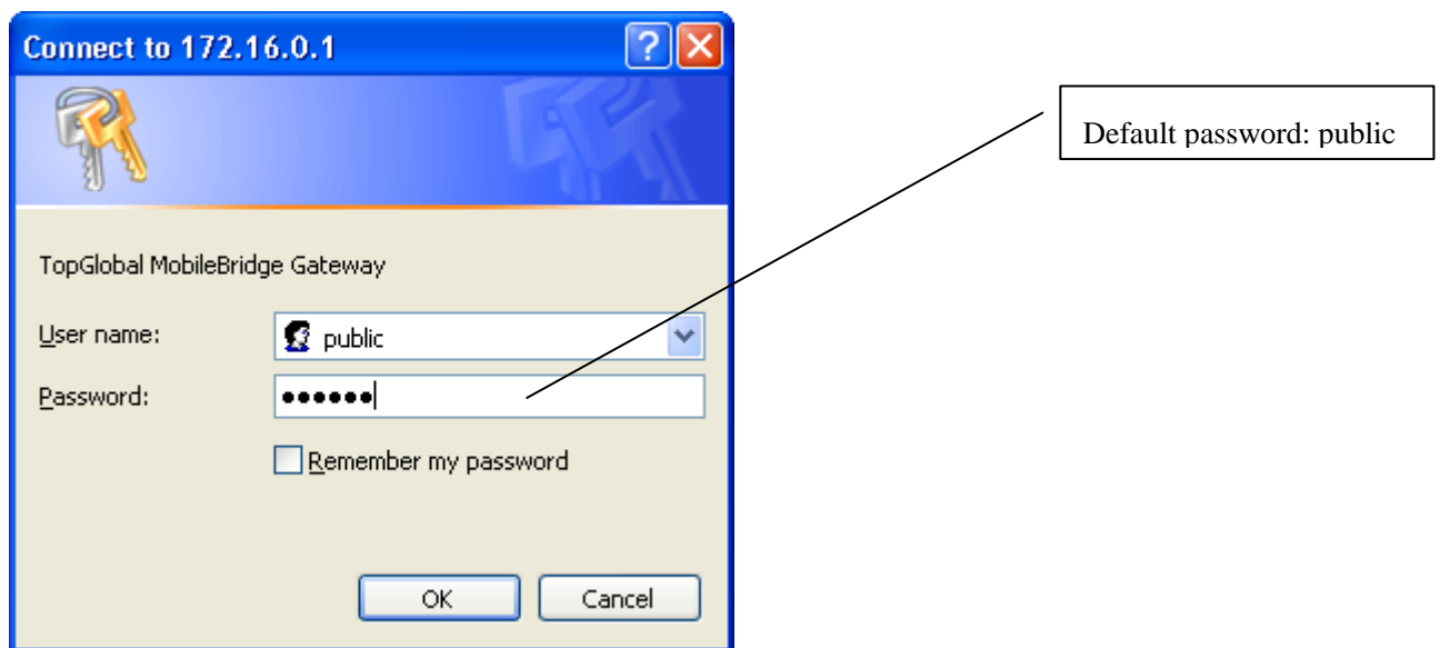
Figure 2-3 Login windows
