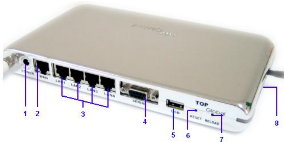
Figure 2-2 Ports description
